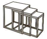
250 (1) H 580, 550, 530 L 440, 420, 400 B 340, 290, 240
